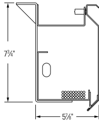
Cross Sectional View of Power Raceway
